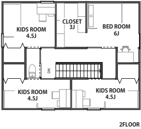
2FLOOR
