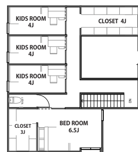
2FLOOR
