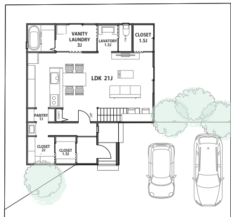
1FLOOR
